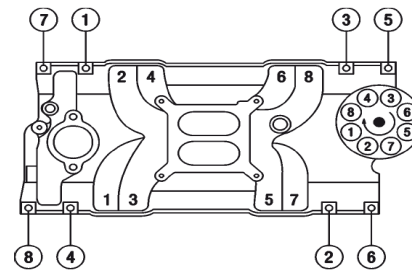
FIRING ORDER 1-8-4-3-6-5-7-2
